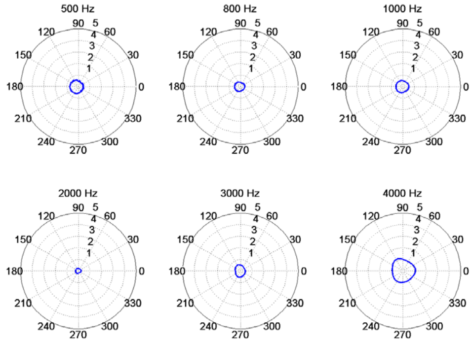
Figure 3.13. Directivity plots for the absolute value of the intensity magnitude error for the PA array.
