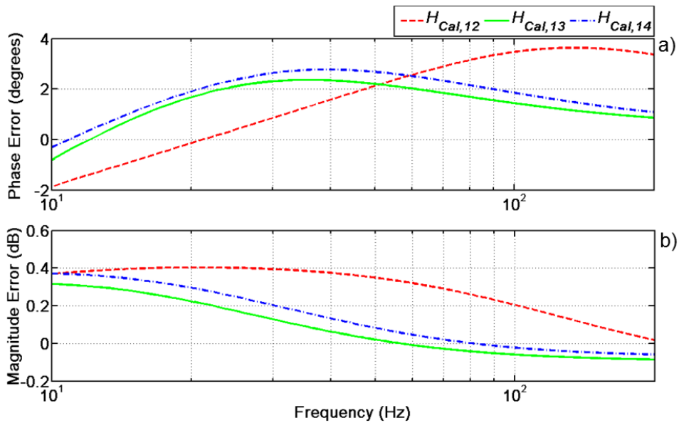
Figure 2.7. Phase (a) and magnitude (b) transfer functions for the microphones used in the experimental array.
