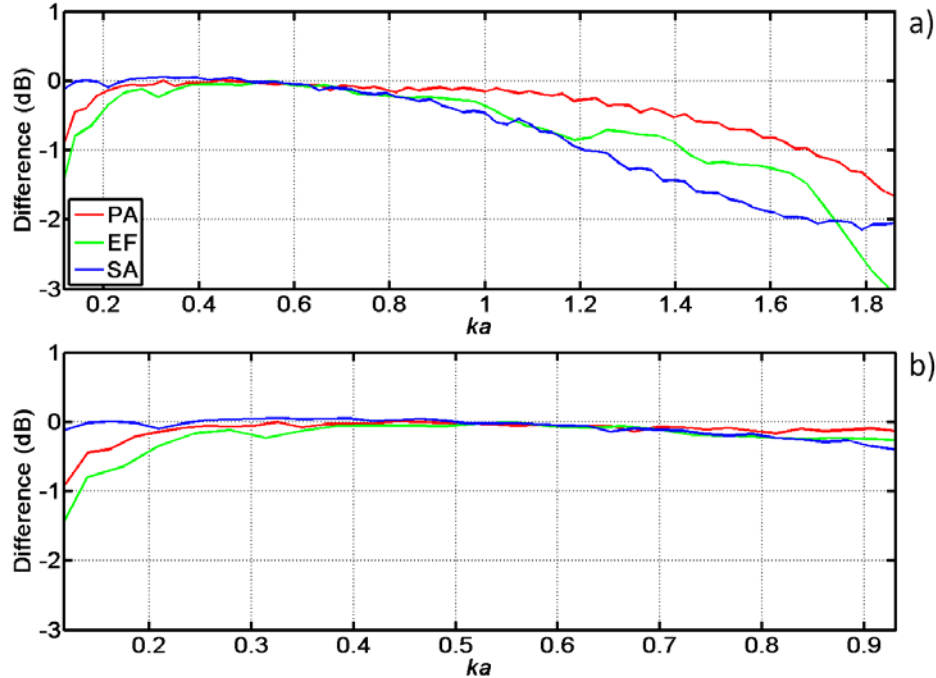
Figure 4.7. Difference between sound intensity level and sound energy density level for the PA, EF and SA arrays for a) 500 Hz to 8 kHz and b) 500 Hz to 4 kHz assuming a=1.27 cm.
